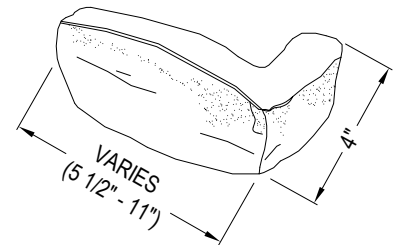
90° CORNER DETAIL
