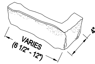
90° CORNER DETAIL
