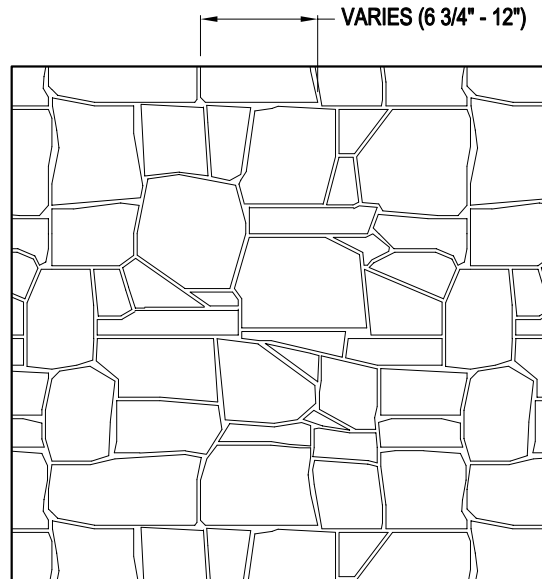
PATTERN - SANDSTONE
