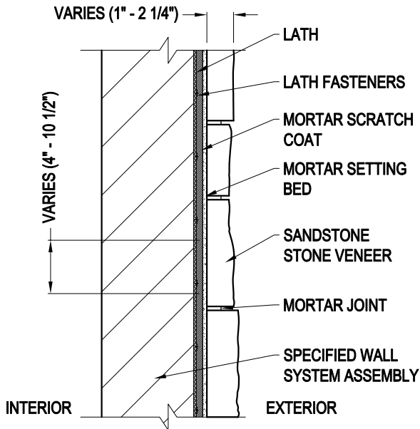
TYPICAL SECTION
