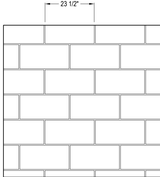
PATTERN - CASTSTONE
