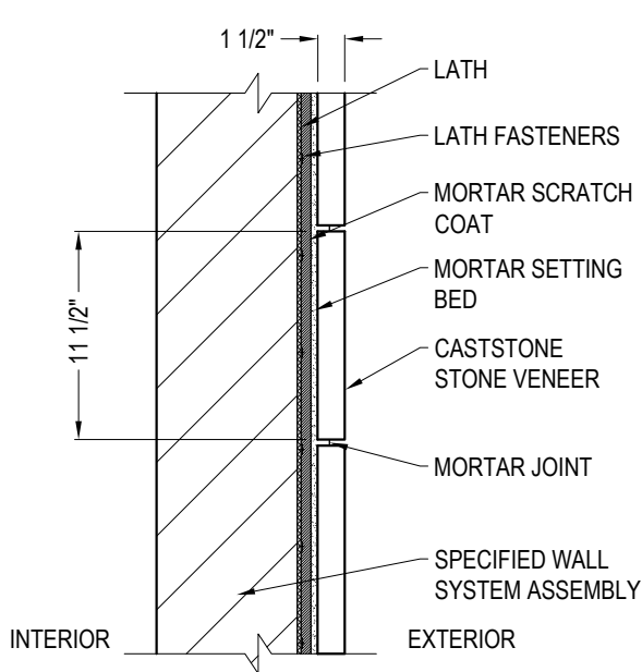
TYPICAL SECTION
