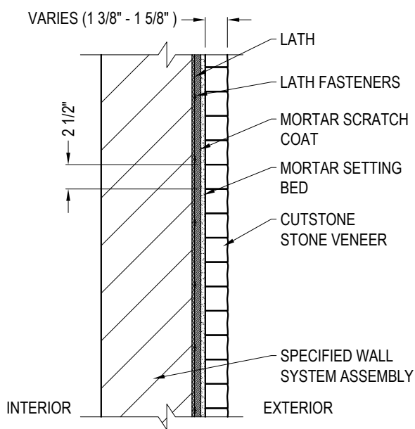
TYPICAL SECTION
