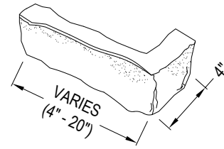
90° CORNER DETAIL
