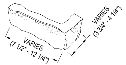
90° CORNER DETAIL
